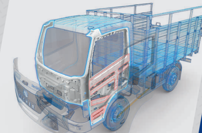
Dual panel cabin adapted from Japanese design
